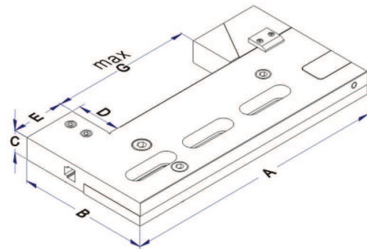
Installation illustration
